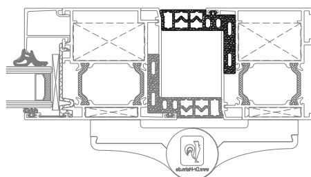
Joint anti-pince doigt
